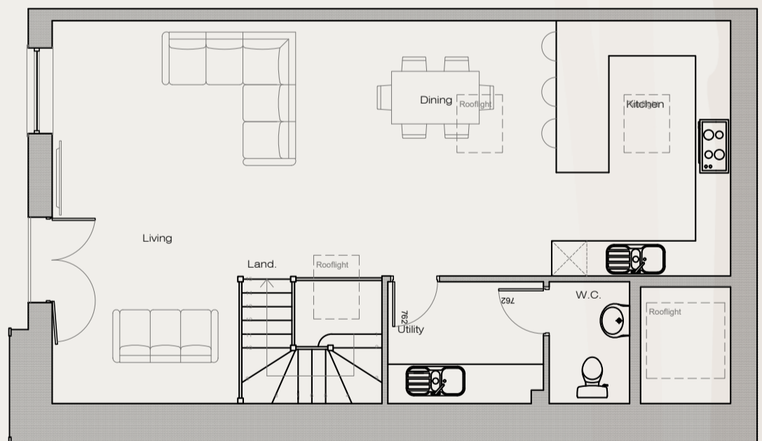
Second Floor Level
