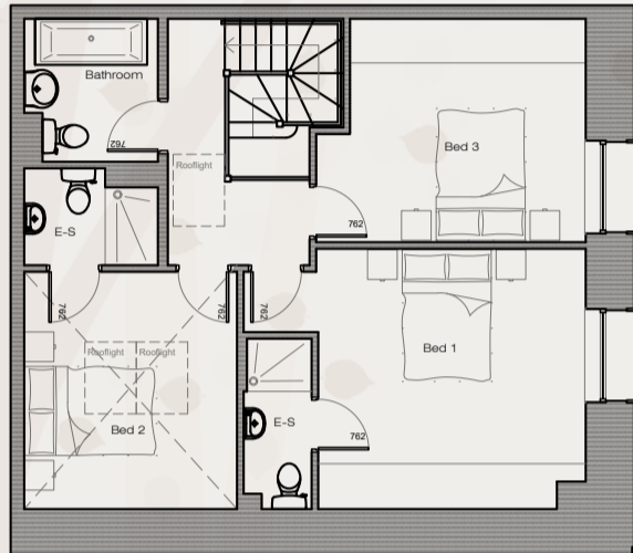
Second Floor Level
