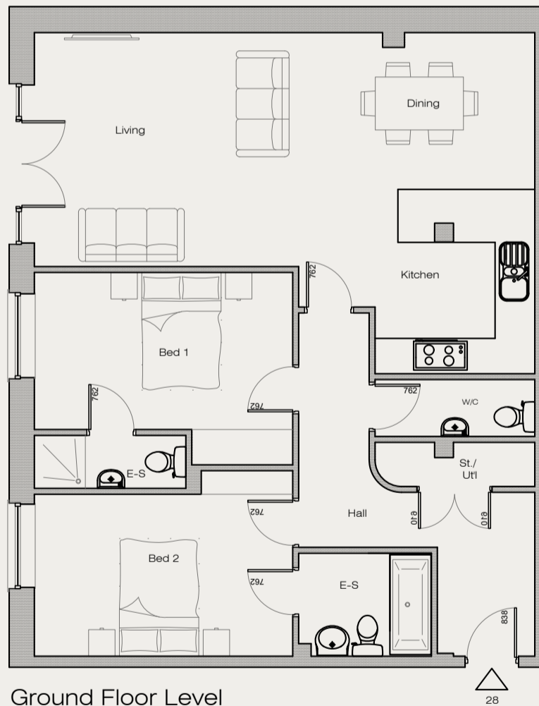
Apartment Entrance Floor Level - Ground Floor
