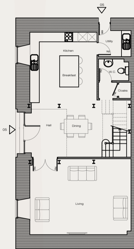
Lower Ground Floor Level
